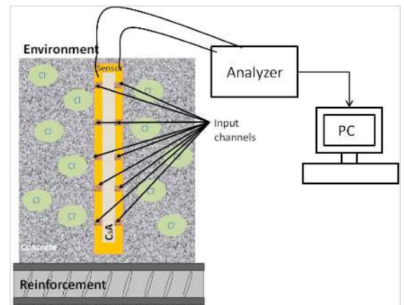
Figure 5.2: Sensor location
